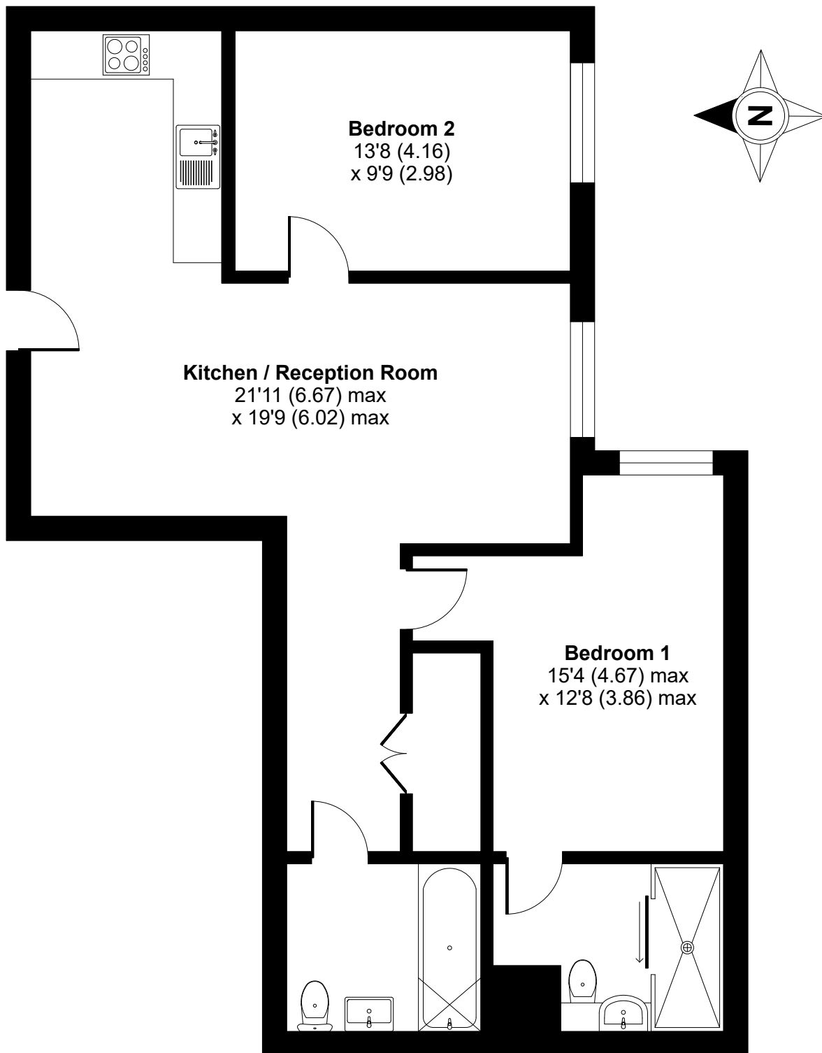
FIRST FLOOR
